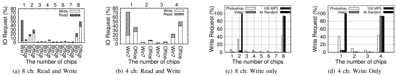
Fig. 11. Channel Parallelism in Page Mapping
