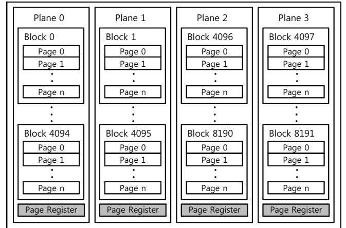
Fig. 1. Structure of NAND Flash Memory [19]
