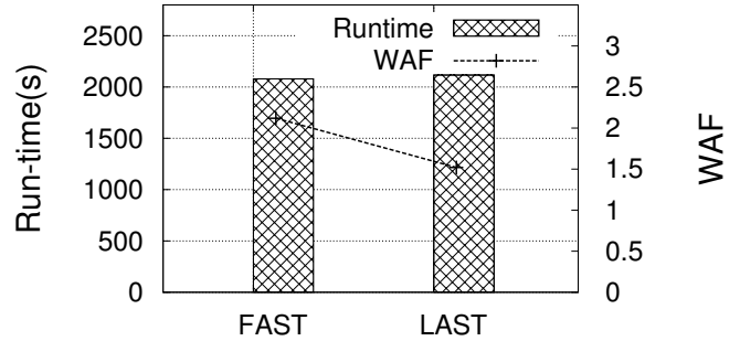
Fig. 13. Write Amplification and Performance (Windows 7 Installation)
